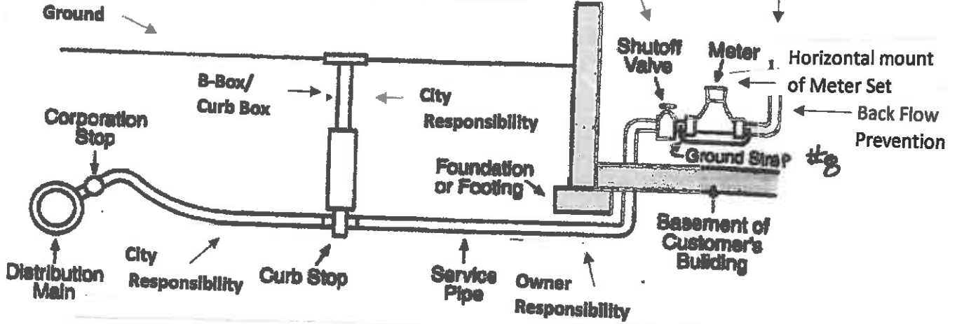
Service Connection with meter in a residence or business
